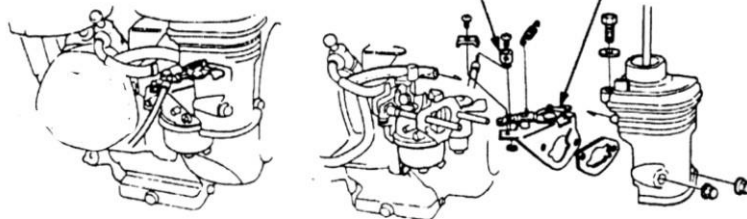
Remote-controlled choke
